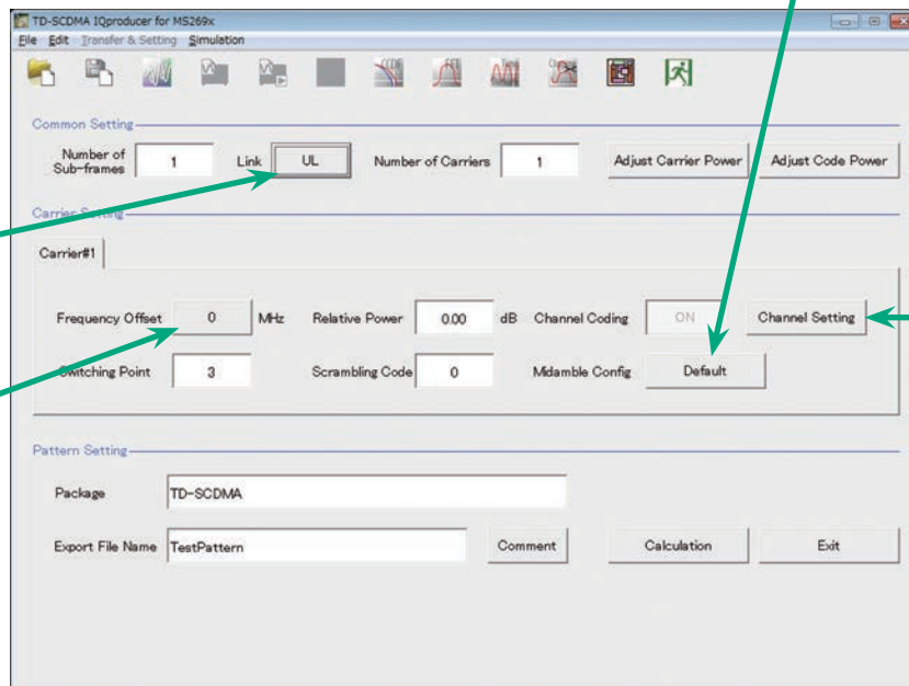
TD-SCDMA IQproducer Setting Screen
