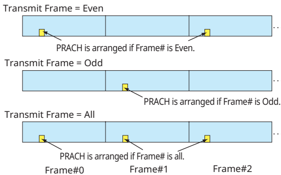
Configuration of PRACH Frame according to Transmit Frame
