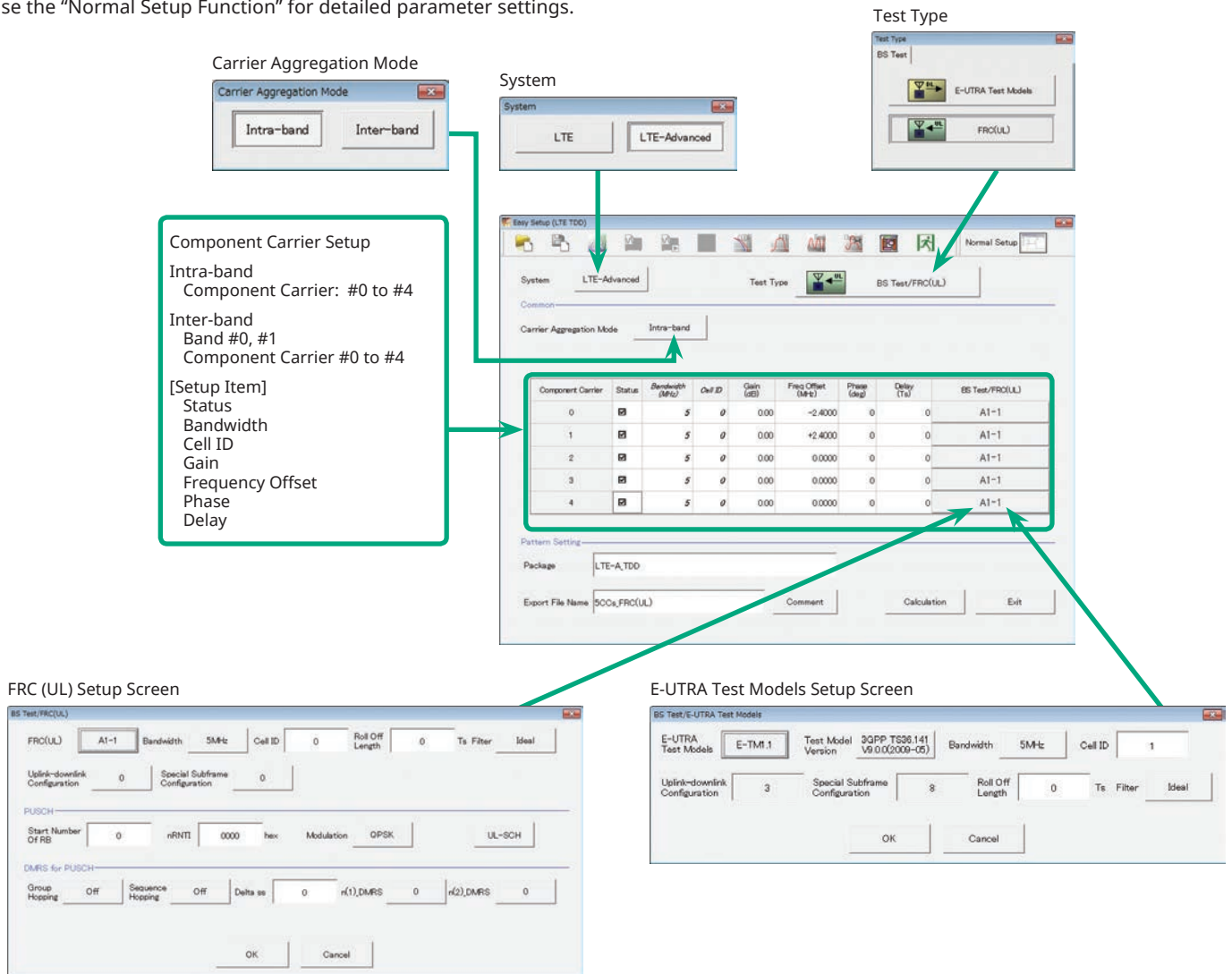
LTE-Advanced Easy Setup Screen (Example: FRC (UL))
