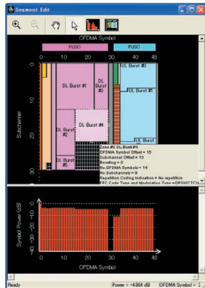
Segment Edit Screen
