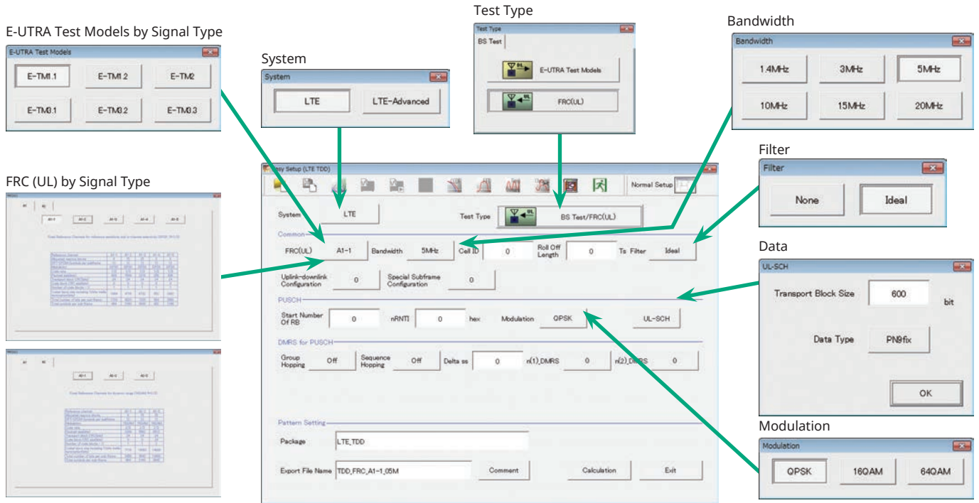
Easy Setup Screen (Example: FRC_UL)
